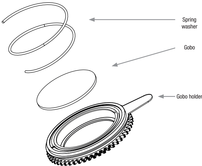
Gobo holder for rotating gobos
